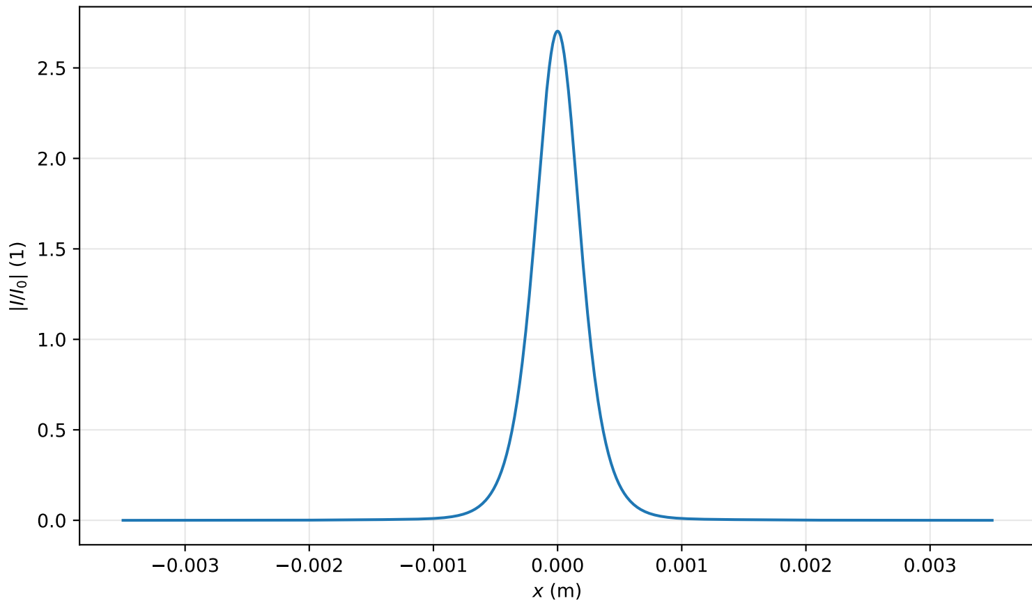
Intensity profile I(x, y = 0, z = 3.105m)/I_0 , P_{in}=1.0P_{cr} , artificial time
